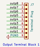
Output Terminal Block 1
